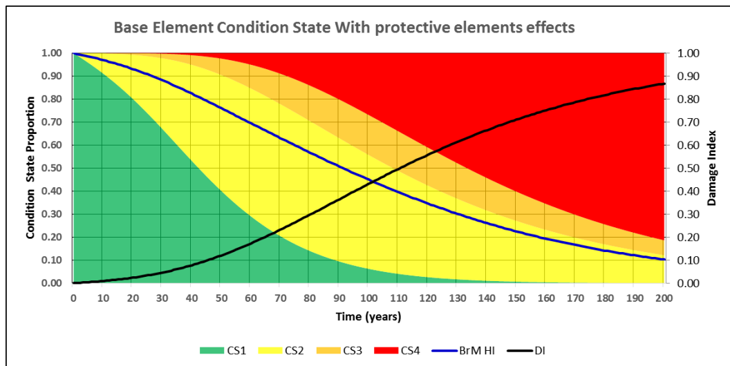
Markovian Model or \beta=1
