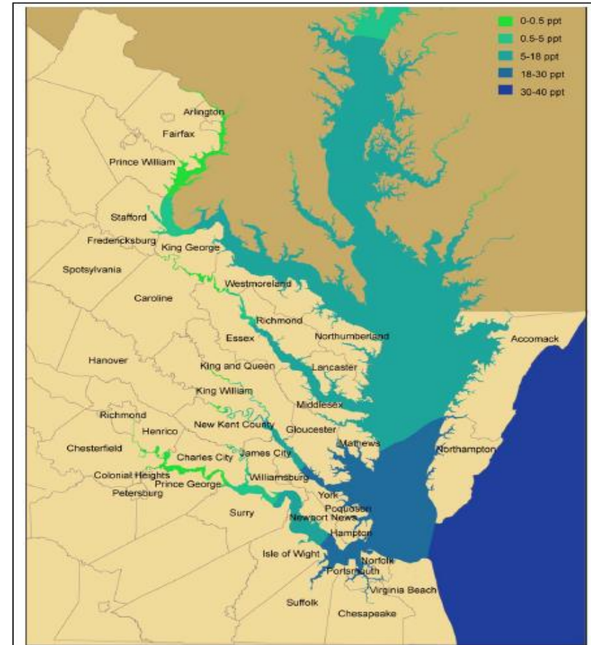
Figure 4. General Salinity Distribution in Virginia
