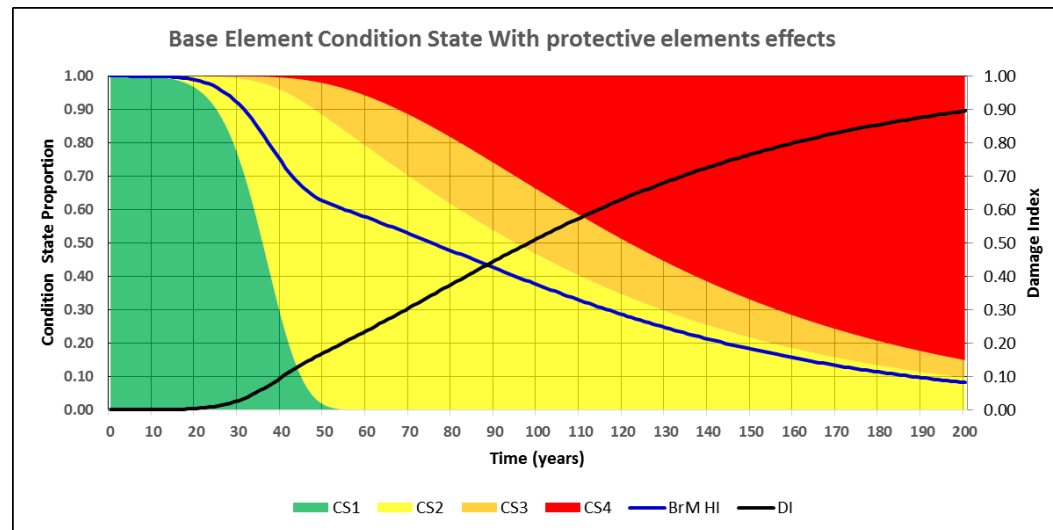
Weibull Model \beta=3
